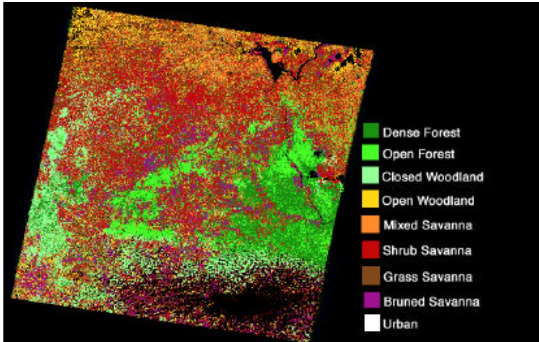
Figure 4. Classification of the Landsat TM image (path 185, row 56). The overall accuracy of classification is 92% with dense forest 94%, open forest 86%, closed woodland 89%, open woodland 93%, mixed savanna 78%, shrub savanna 83%, grass savanna 97%, burned savanna 98%, and urban 88%.
