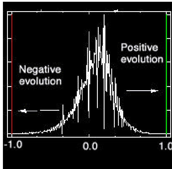
Figure 8. Histogram of the change image based on the normalized difference between the 2000 and 1989 MSAVI images. The arrows indicate the modified pixels and the threshold were fixed at \pm 1 standard deviation.
