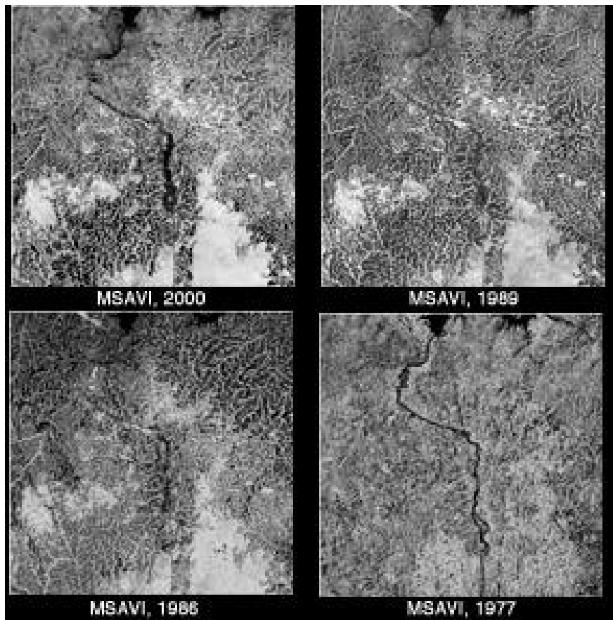
Figure 6. Changes in vegetation cover from 1977 to 2000 as demonstrated by MSAVI. The loss of ecotone vegetation due to savanna burning and agricultural practices can be observed in lower left corner of the images. The upper left corner of the images shows vegetation loss up to 1989 and woody encroachment from 1989 to 2000.
