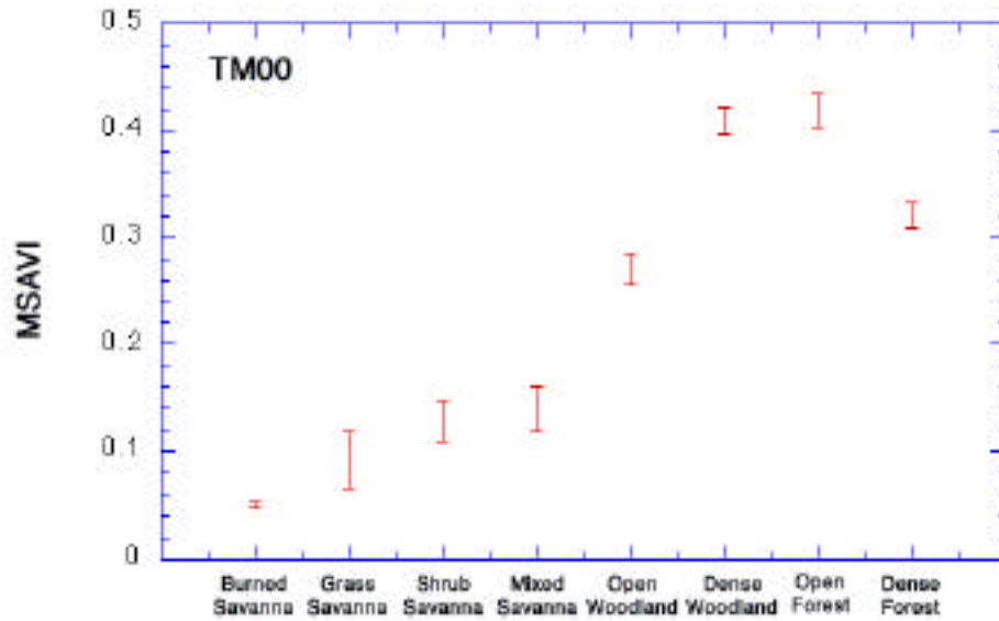
Figure 7. Mean and standard deviation of MSAVI signatures of vegetation types. Except for grass and shrub savanna, MSAVI can differentiate vegetation types.
