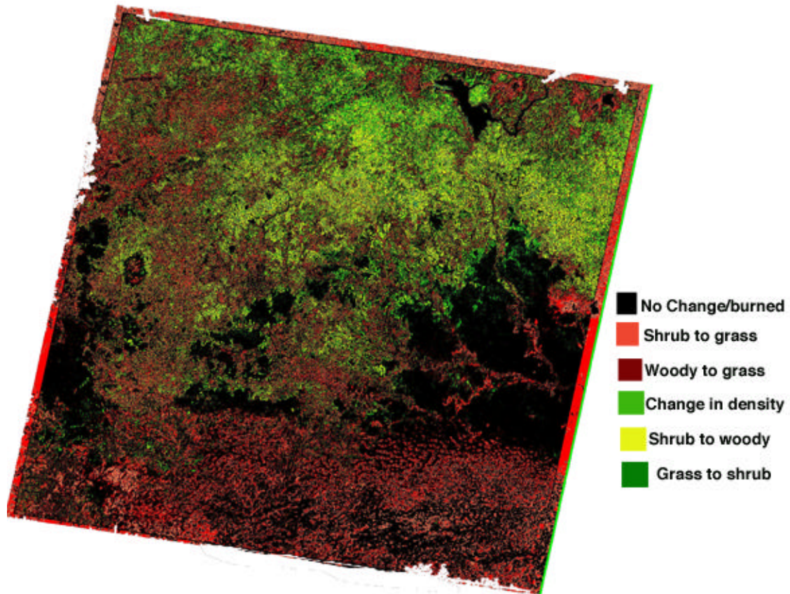
Figure 9. Land cover change map showing the evolution of vegetation types between 1989 and 2000. The dark areas represent no change between two dates regardless of the land cover type.
